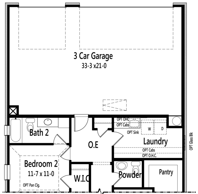
OPT 3-Car-Garage
