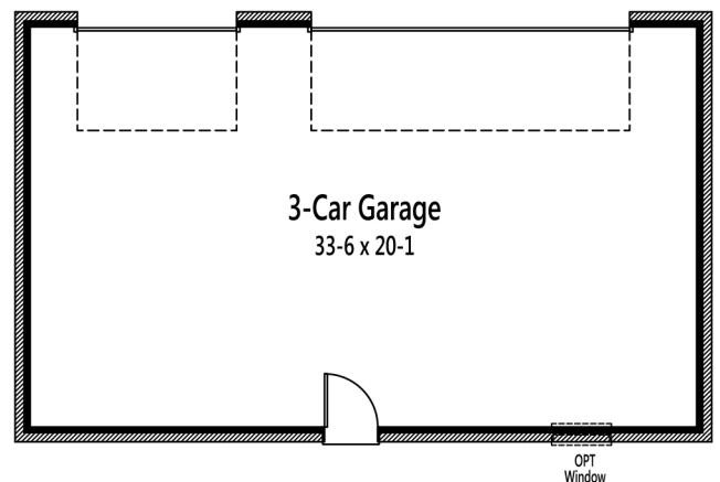
OPT 3-Car-Garage
