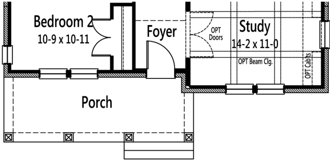
Texana Farmhouse Brick With OPT Porch
