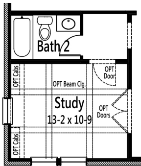
OPT Study ILO Bedroom 2
