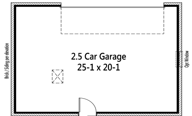
OPT Detached 2.5-Car-Garage
