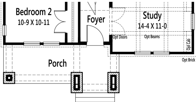
Main Floor Craftsman with OPT Porch
