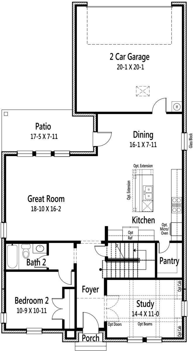
Main Floor European Romantic
