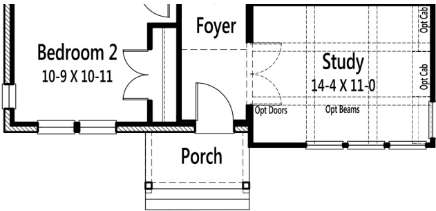
Main Floor Modern
