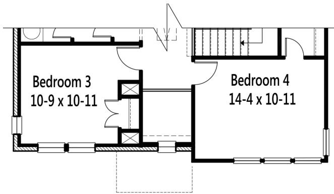
Upper Floor Modern
